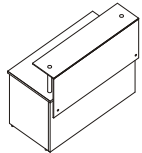
AT.RCM.08.65 - 800X650X1100 AT.RCM.09.65 - 900X650X1100 AT.RCM.10.65 - 1000X650X1100 AT.RCM.12.65 - 1200X650X1100 AT.RCM.14.65 - 1400X650X1100 AT.RCM.16.65 - 1600X650X1100 AT.RCM.18.65 - 1800X650X1100
