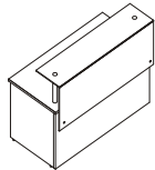
AT.RCM.08.65 - 800X650X1100 AT.RCM.09.65 - 900X650X1100 AT.RCM.10.65 - 1000X650X1100 AT.RCM.12.65 - 1200X650X1100 AT.RCM.14.65 - 1400X650X1100 AT.RCM.16.65 - 1600X650X1100 AT.RCM.18.65 - 1800X650X1100
