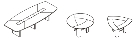
PR.REU.26.12 - 2600x1200x740 PR.REU.31.13 - 3100x1300x740 PR.REU.36.14 - 3600x1400x740 PR.REU.41.15 - 4100x1500x740 * outras dimensões sob consulta
